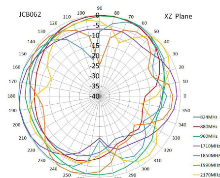
Radiation Pattern (GSM XZ)
