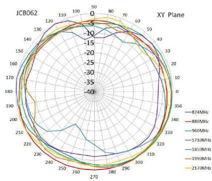
Radiation Pattern (GSM XY)
