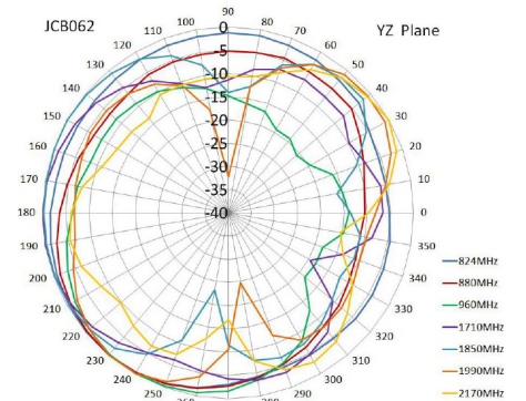
Radiation Pattern (GSM YZ)
