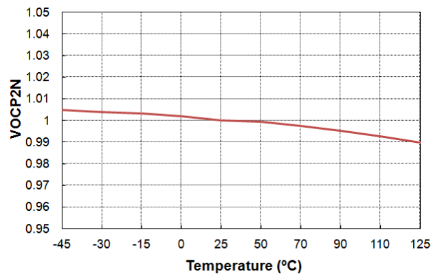
Figure 50. V_{OCP2N} vs. Temperature
