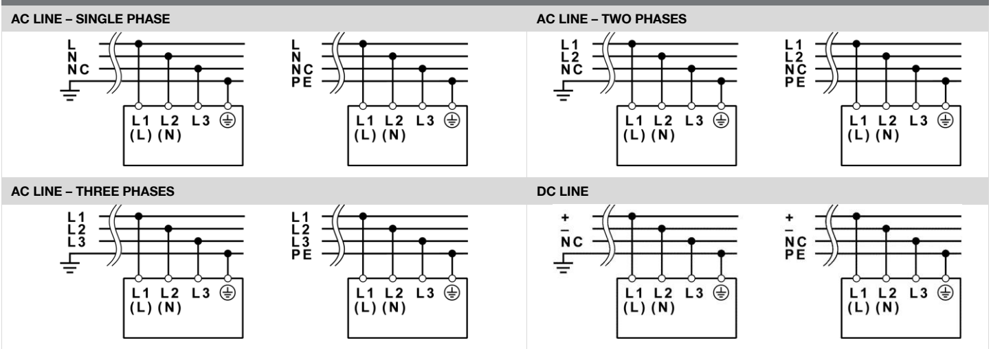
FIG.7 - INPUT CONNECTIONS
