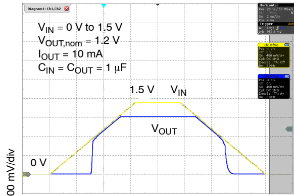
2 ms/div Figure 36. Turn On/Off, Slow Rising V IN
