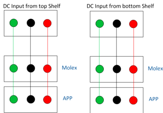
Figure 1: Electrical Schematic
