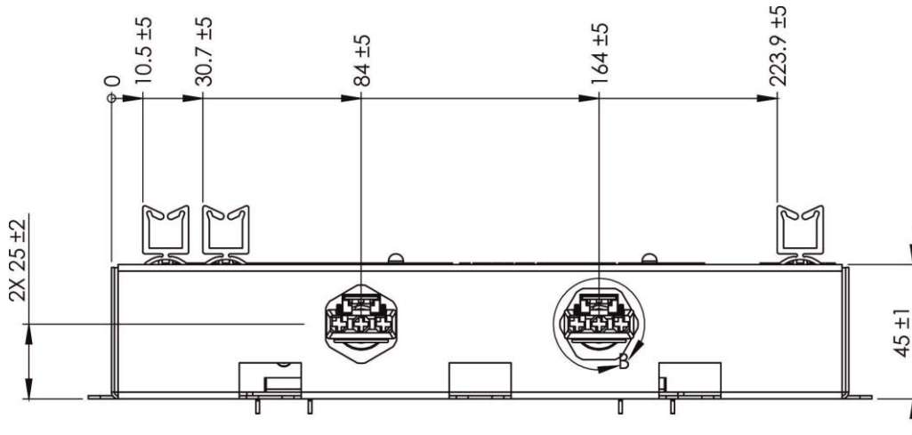
Figure 7. Dimension Drawing DC PDU (Side View)
