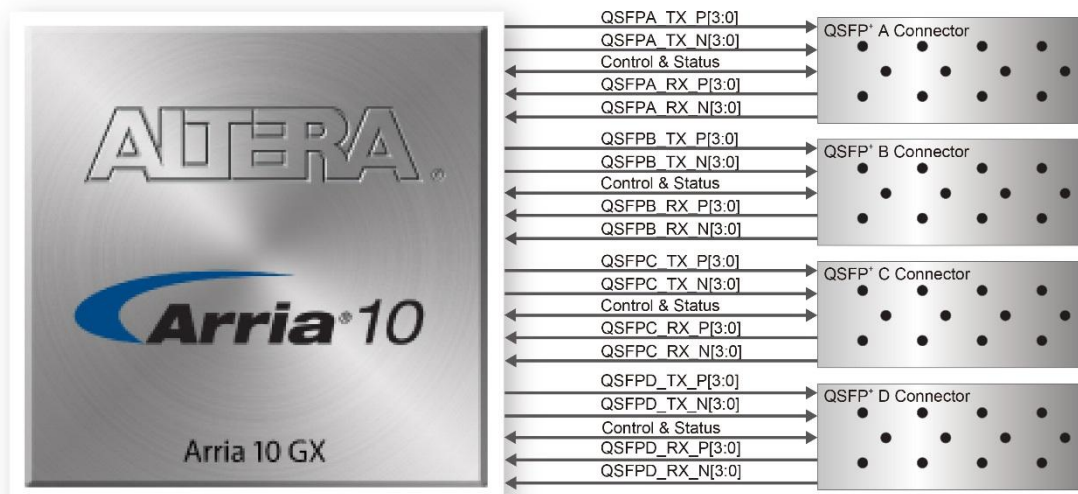
Figure 2-12 Connection between the QSFPA and Arria GX FPGA
