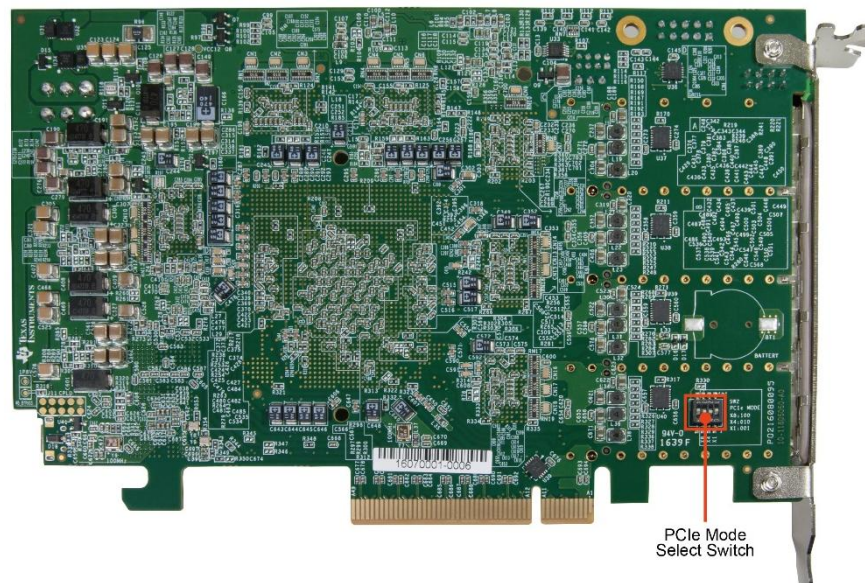
Figure 2-2 FPGA Board (Bottom)
