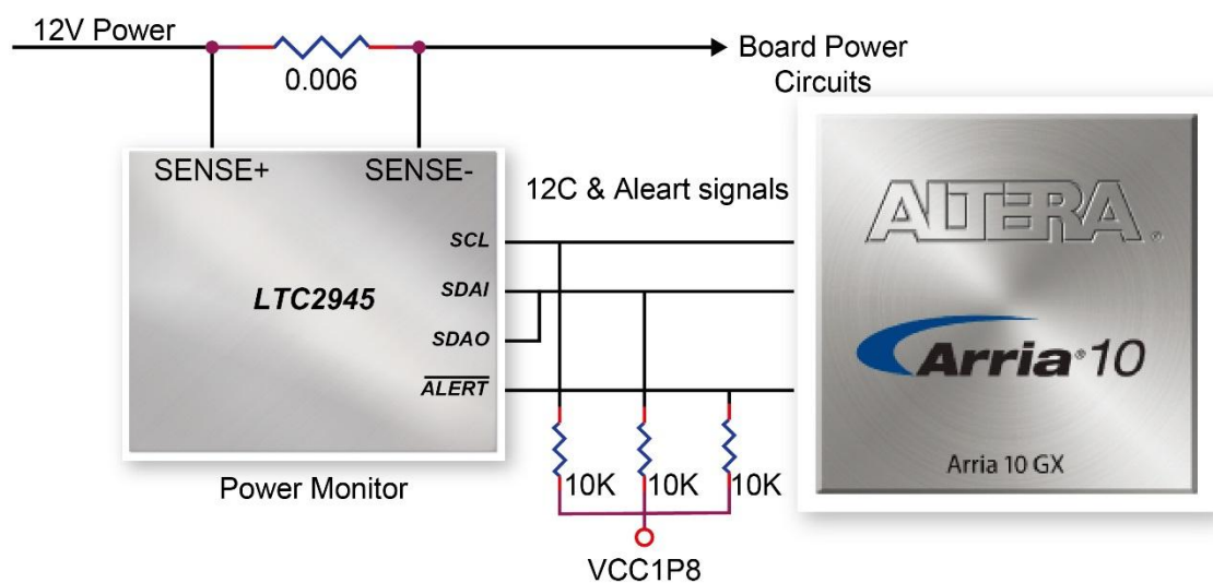
Figure 2-9 Connections between the Power Monitor chip and the Arria 10 GX
