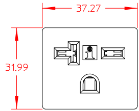
8825100 & 88252100 QUICK DISCONNECT CONTACTS
