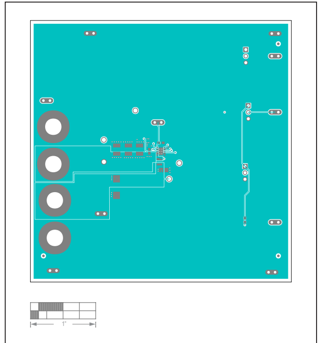
MAX20474 EV Kit PCB Layout—Top Layer
