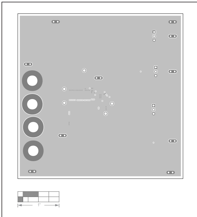
MAX20474 EV Kit PCB Layout—Layer 2
