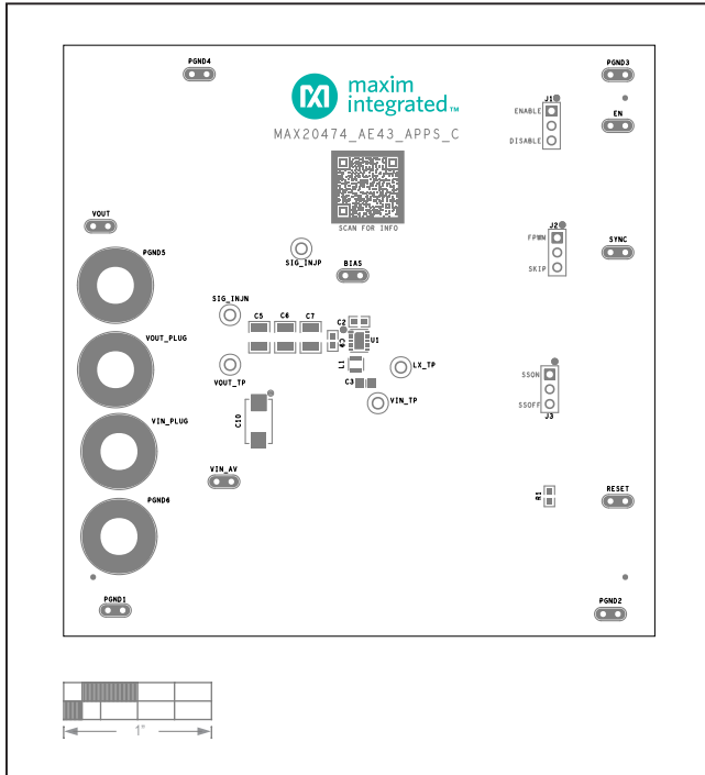
MAX20474 EV Kit PCB Layout—Top Silkscreen
