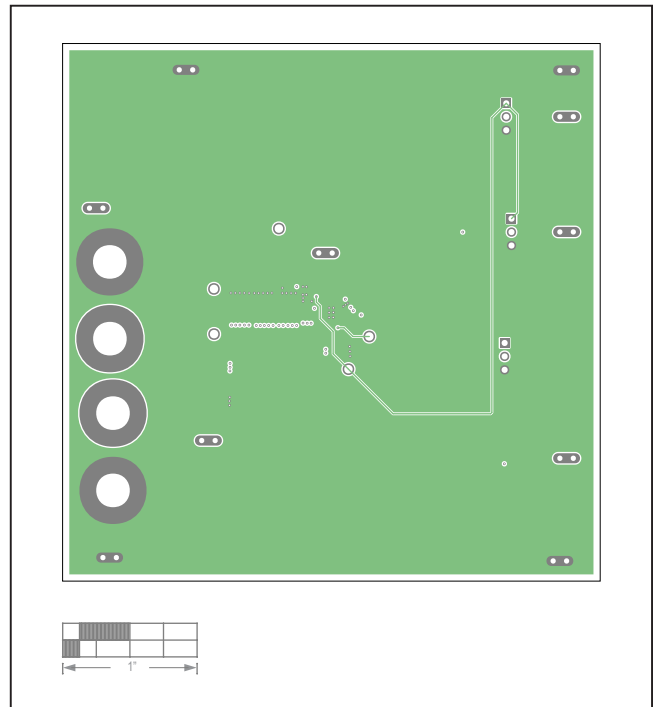
MAX20474 EV Kit PCB Layout—Layer 3
