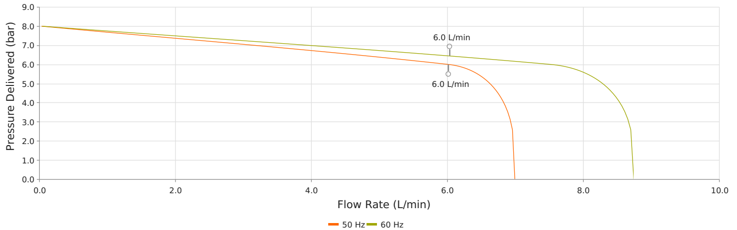
WL5000 - Pump Curve
