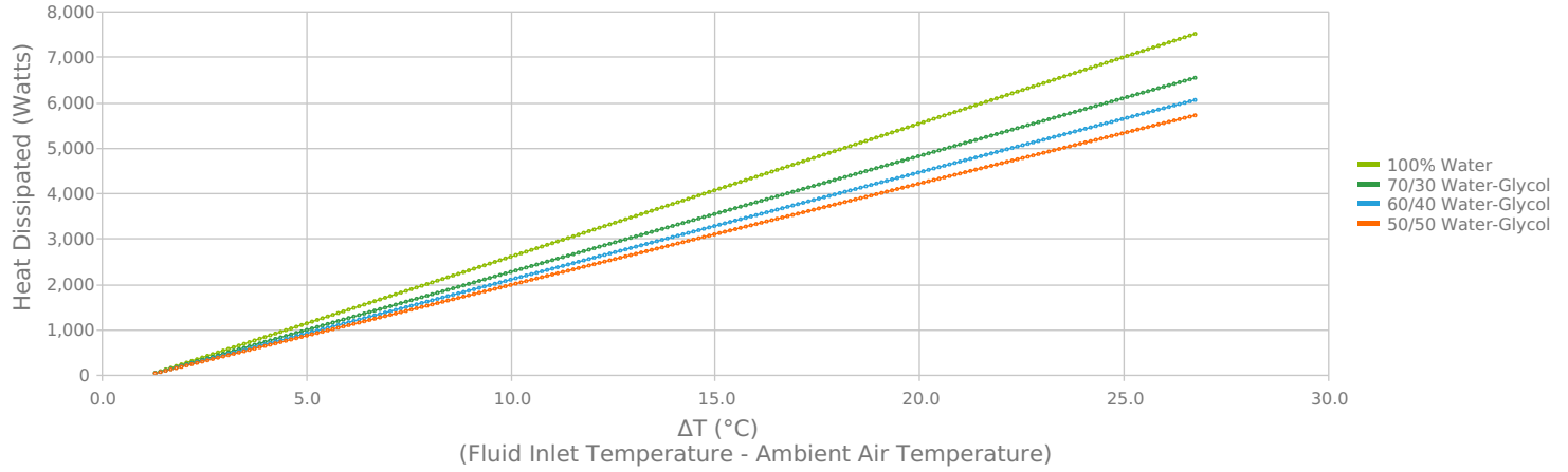
WL5000 Fluid Inlet/Outlet Temperature Difference (ΔT) @ Nominal Flow 6 L/min
