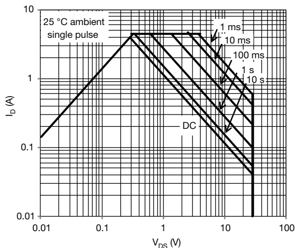
Fig. 33 - SOA on Application Board
