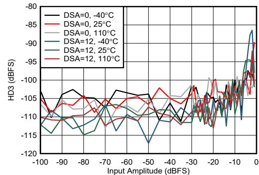
Figure 6-225. RX HD3 vs Input Amplitude at 6.851GHz
