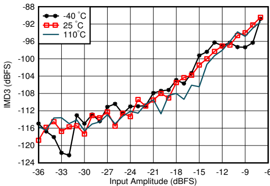
Figure 6-97. RX IMD3 vs Input Level and Temperature at 1.75 GHz
