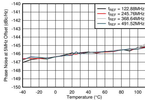
Figure 6-242. Phase Noise for 12-GHz VCO at 5-MHz Offset vs Temperature and f_{REF} at f_{OUT} = 2.6 GHz
