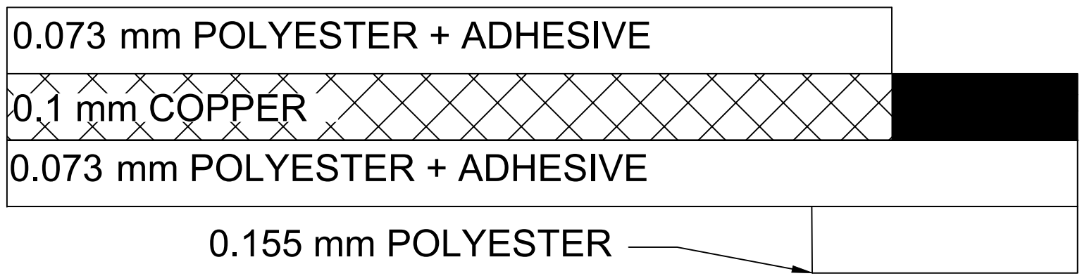
CROSS-SECTION
