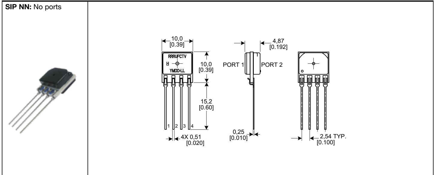
Figure 3. SIP Package Dimensional Drawings (For reference only: mm [in.]
