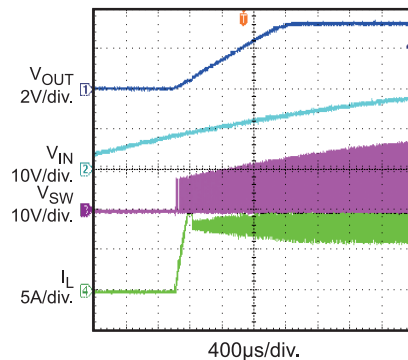
Start Up Through VIN V_{IN} = 22V , I_{OUT} = 8A
