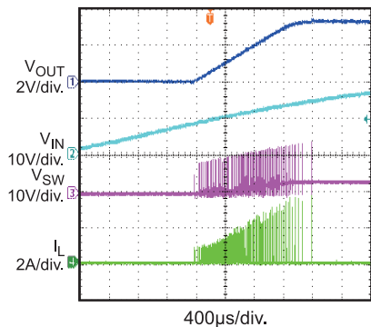
Start Up Through VIN V_{IN} = 22V , I_{OUT} = 0A
