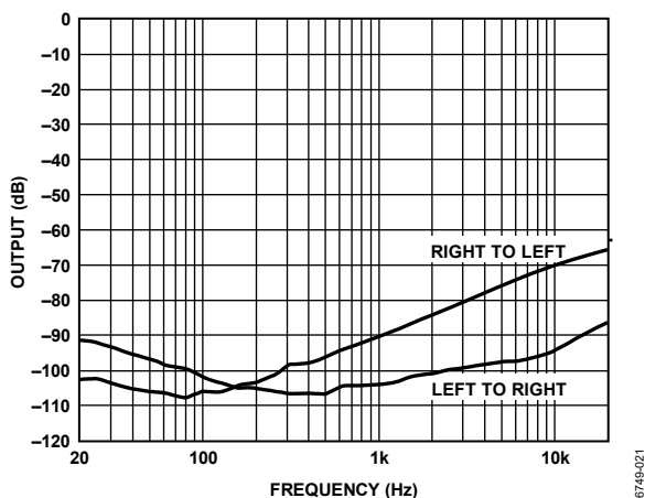
Figure 22. Crosstalk @ 1 W, 6 Ω, PVDD = 15 V, PGA = 0 dB
