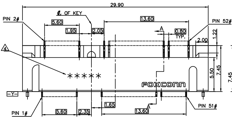
CONNECTOR
