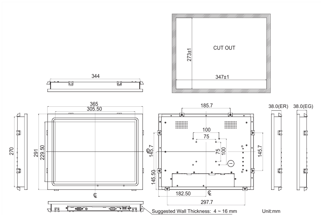
Figure 2.2 IDS-3215E Series Dimensions
