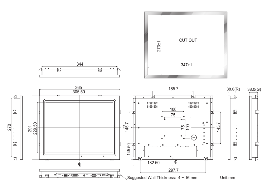
Figure 2.1 IDS-3215 Series Dimensions
