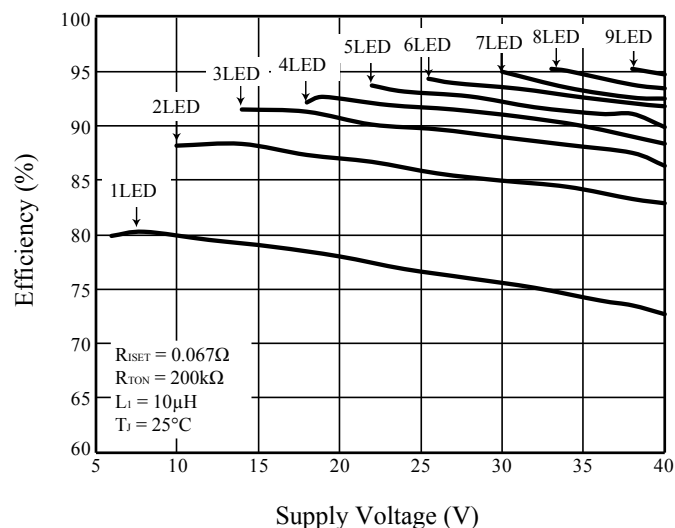
Figure 12 Efficiency vs. V_{CC}
