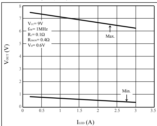
Figure 33 Minimum and Maximum Output Voltage versus LED Current (minimum t_{ON} and t_{OFF} = 150ns)
