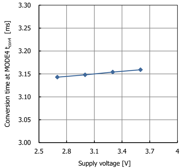
Fig. 22.15 Conversion time at MODE 4 supply voltage characteristic
