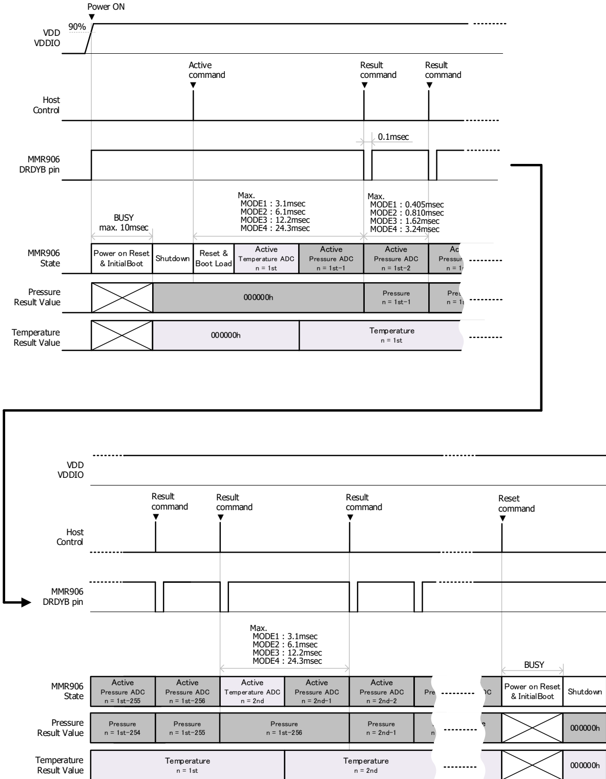
Fig. 8 Timing Chart
