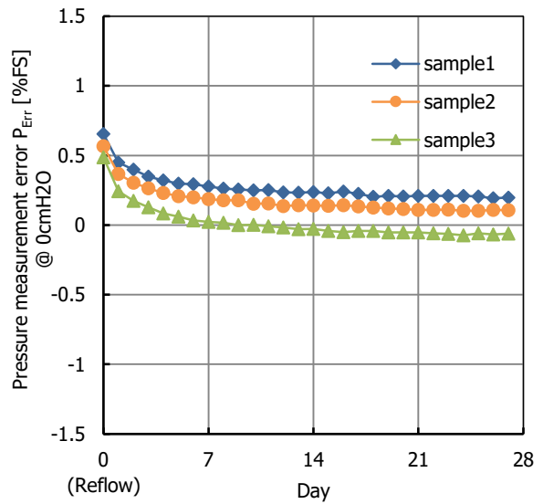
Fig. 22. SEQ22.24Err @0cmH2O Reflow drift
