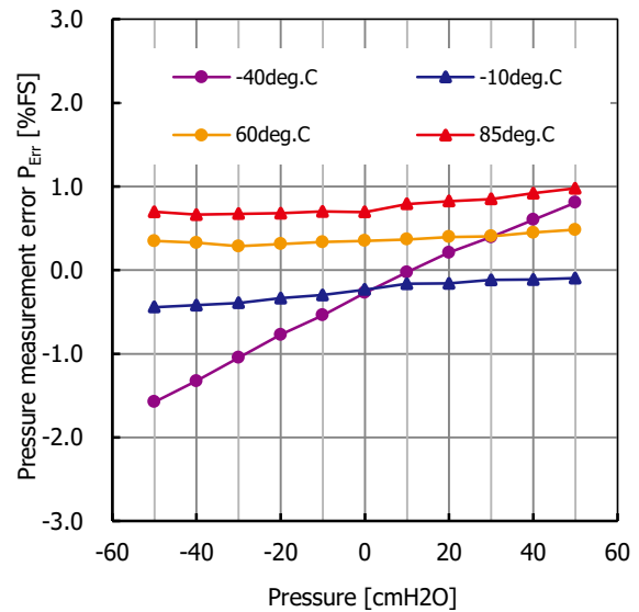
Fig. 22.20 Pressure measurement error P_{Err} temperature characteristic -40~85deg.C
