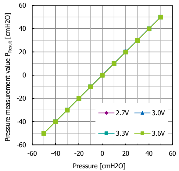
Fig. 22.18 Pressure measurement value P_{Result} supply voltage characteristic
