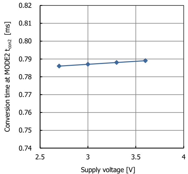
Fig. 22.11 Conversion time at MODE 2 supply voltage characteristic
