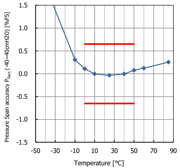
Fig. 22. SEQ22.22 temperature characteristic
