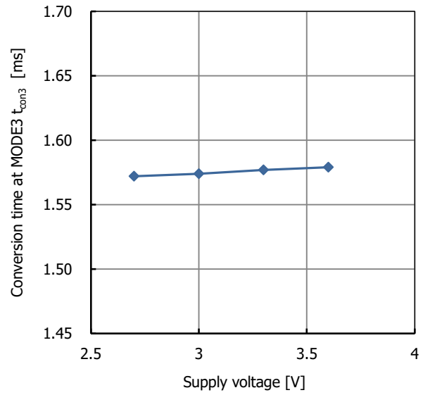
Fig. 22.13 Conversion time at MODE 3 supply voltage characteristic
