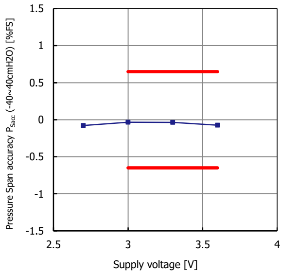
Fig. 22. SEQ22.23 supply voltage characteristic
