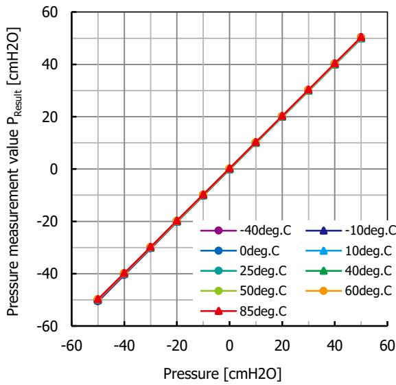
Fig. 22.17 Pressure measurement value P_{Result} temperature characteristic
