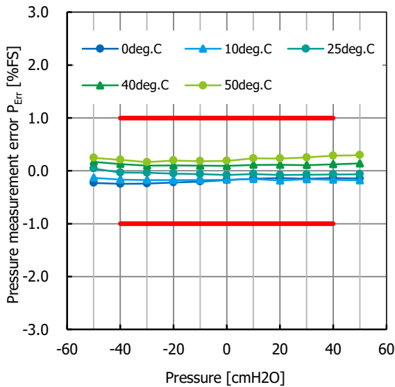
Fig. 22.19 Pressure measurement error P_{Err} temperature characteristic 0~50deg.C
