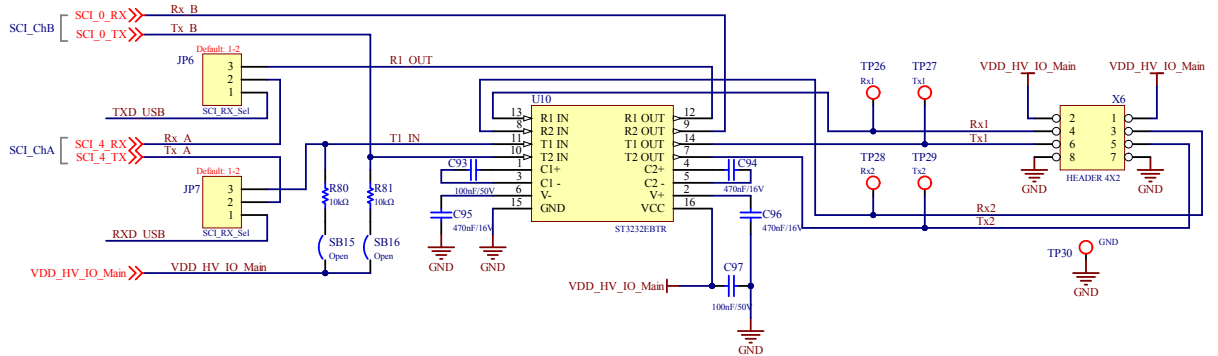
Figure 9. RS232 section
