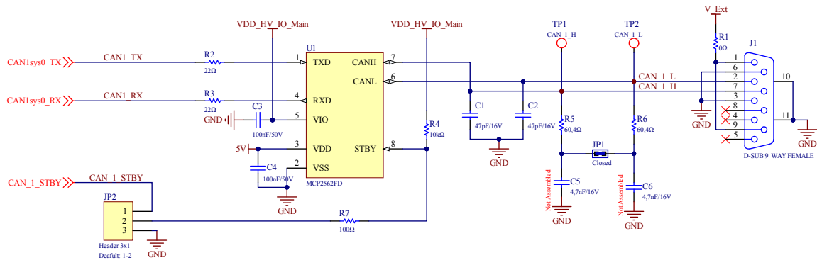
Figure 19. CAN and ISO CAN-FD
