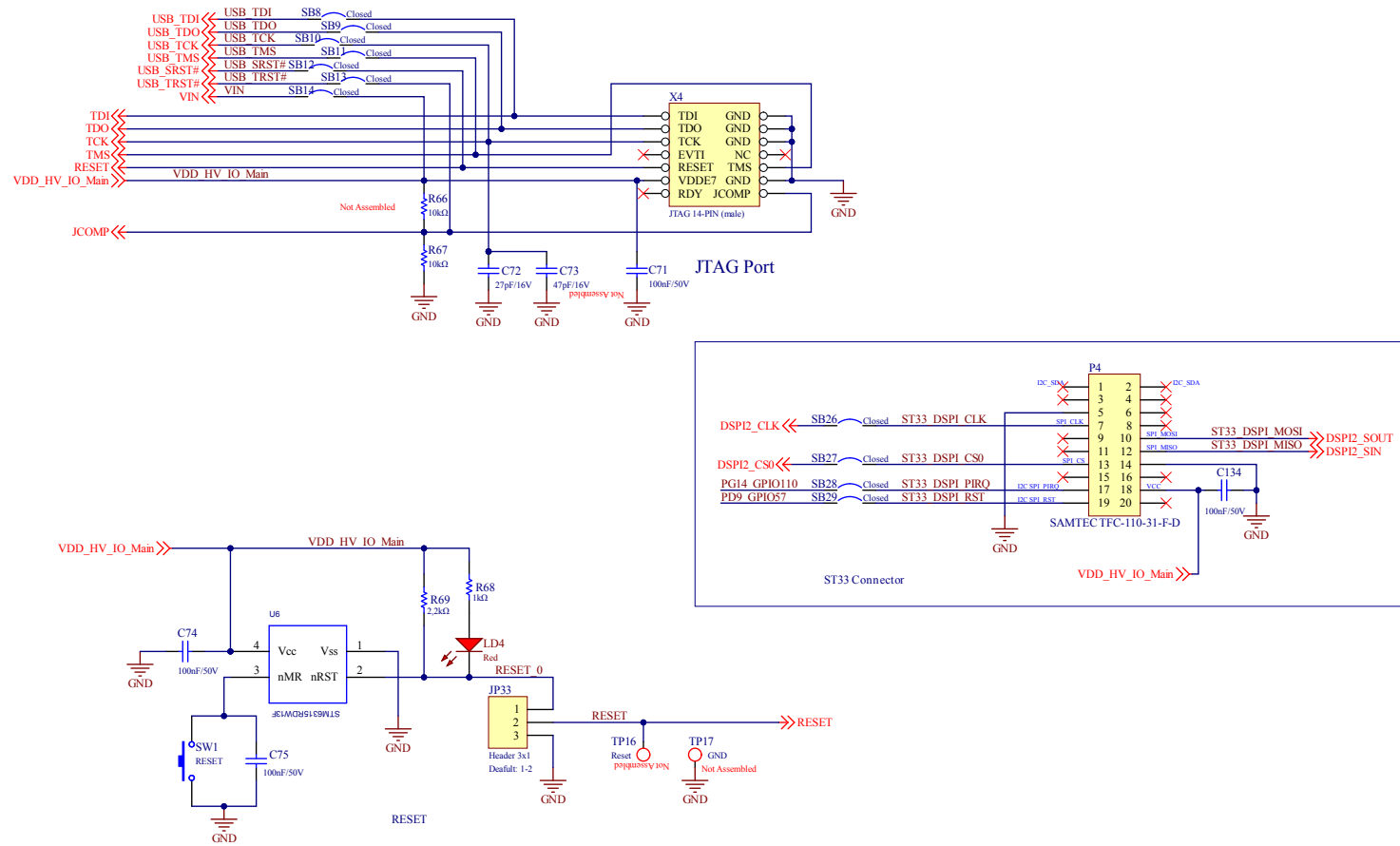
Figure 16. JTAG and reset
