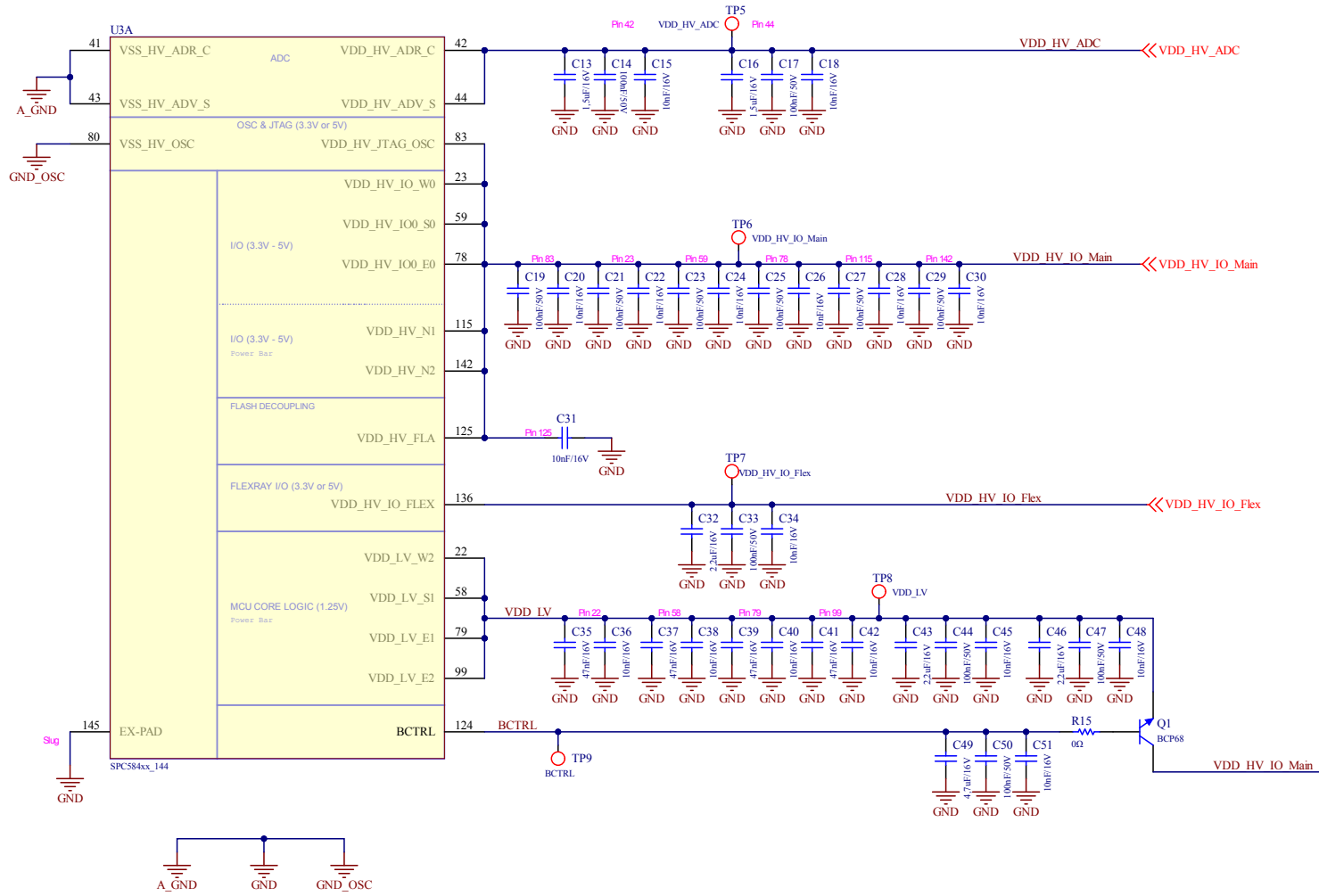
Figure 23. Microcontroller power management
