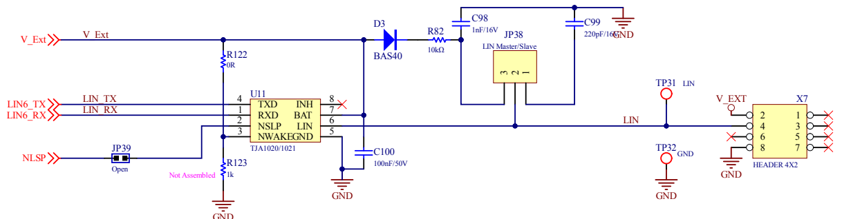
Figure 10. LIN section
