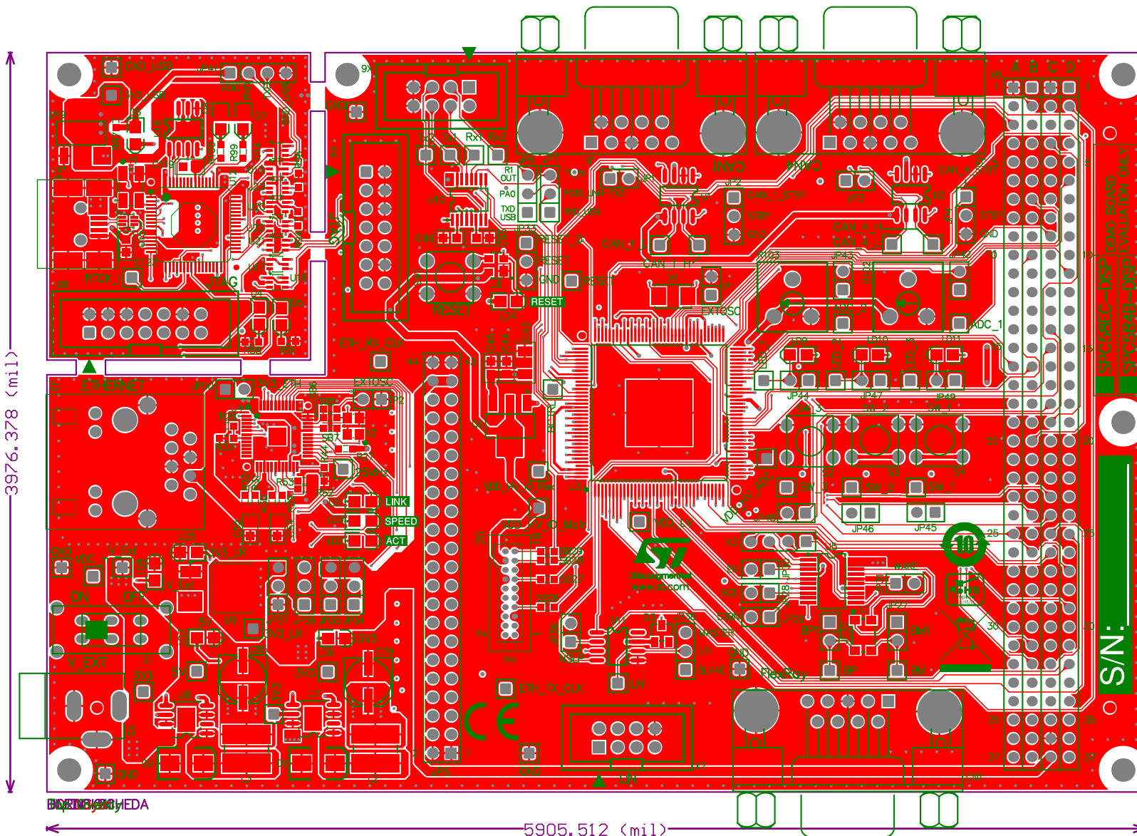
Figure 13. SPC58EC-DISP - PCB top side
