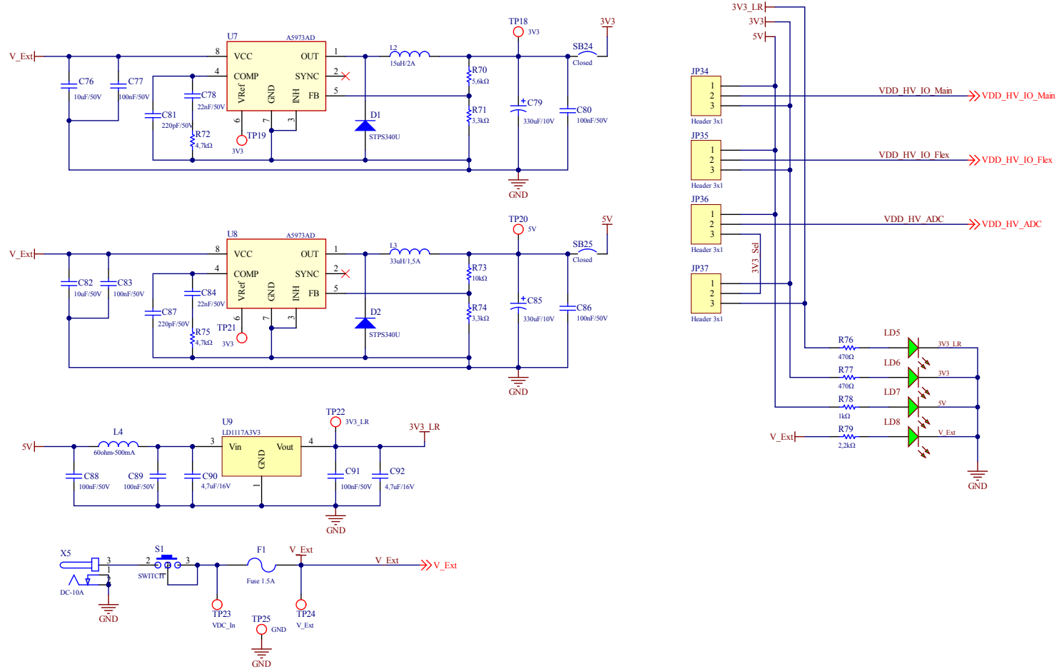
Figure 14. Power supply
