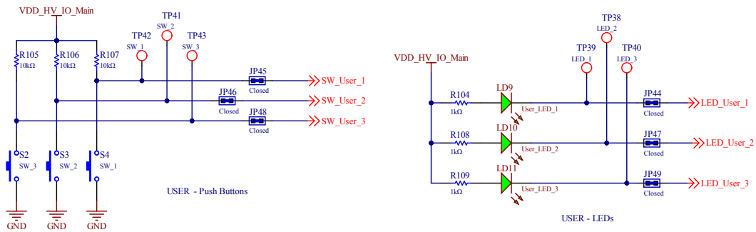
Figure 11. User pushbutton and LEDs
