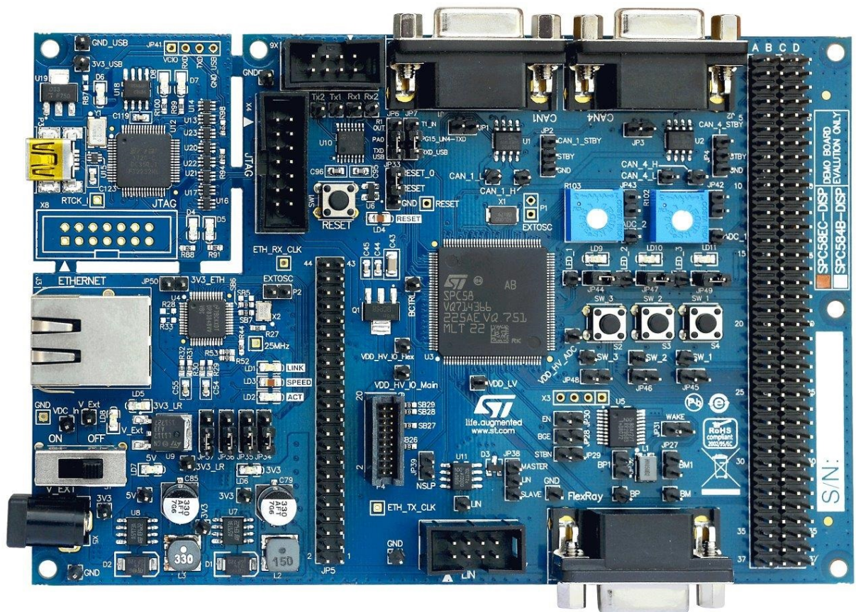
Figure 1. SPC58EC-DISP discovery board-top side
