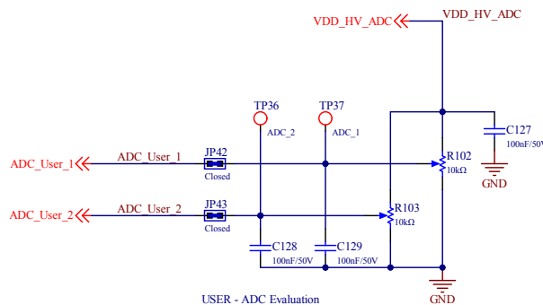
Figure 12. Trimmers
