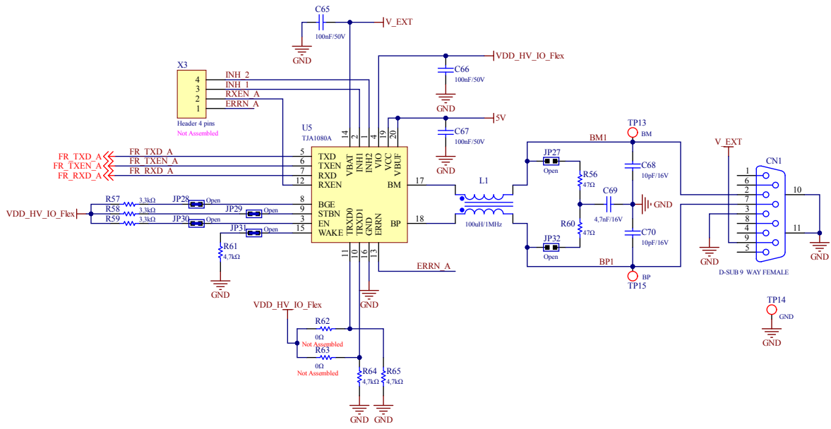
Figure 17. FlexRay
