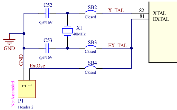
Figure 6. Crystal oscillator
