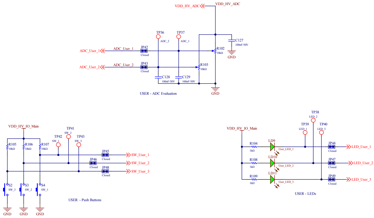
Figure 21. User interface
