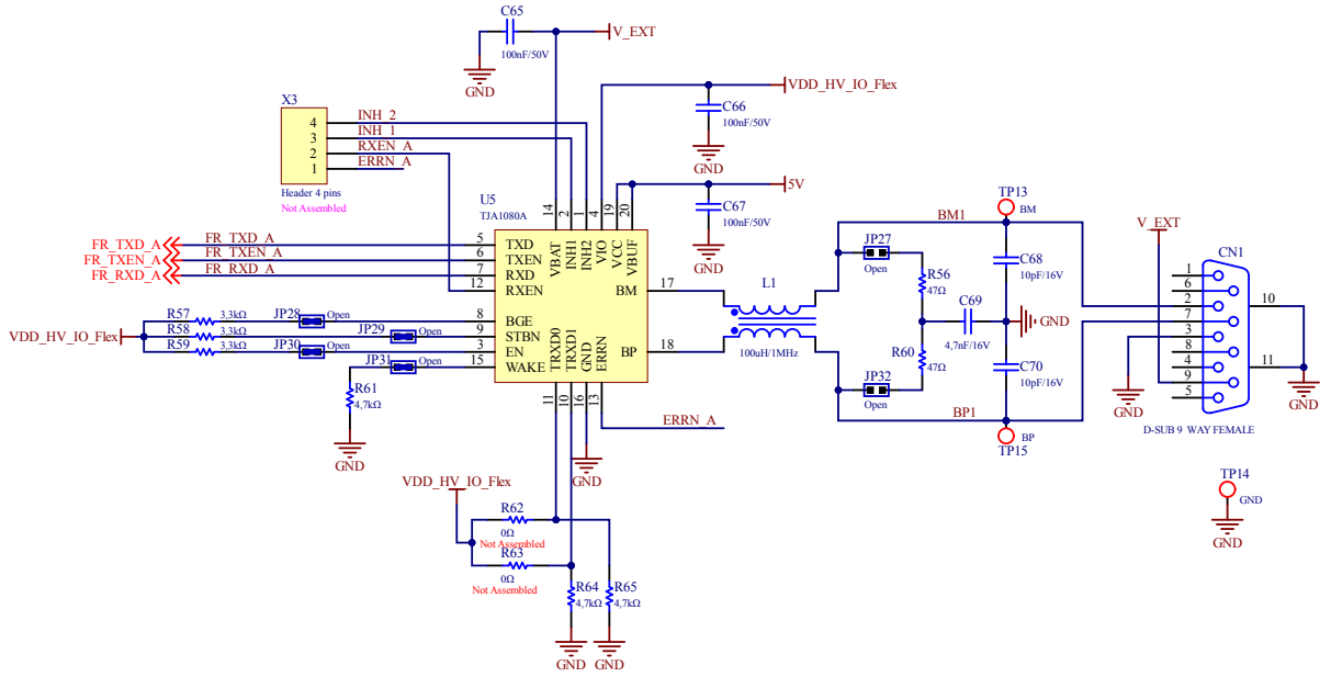
Figure 8. FlexRay
