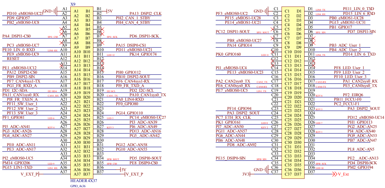
Figure 22. Extended connectors
