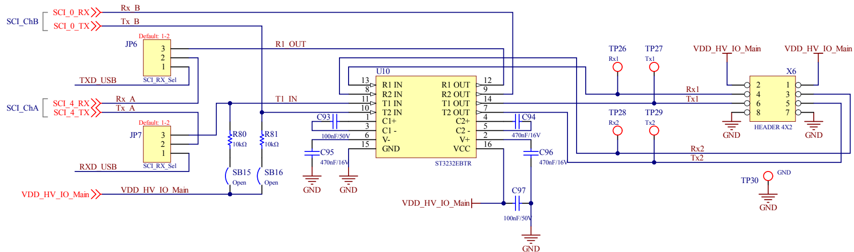
Figure 18. RS232 and LIN
