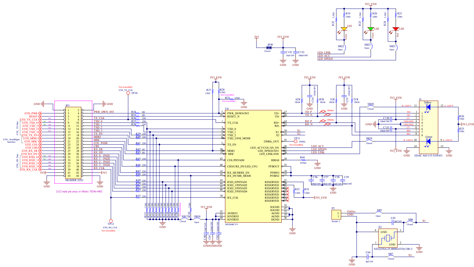
Figure 20. Ethernet
