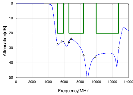
Low band-Port
