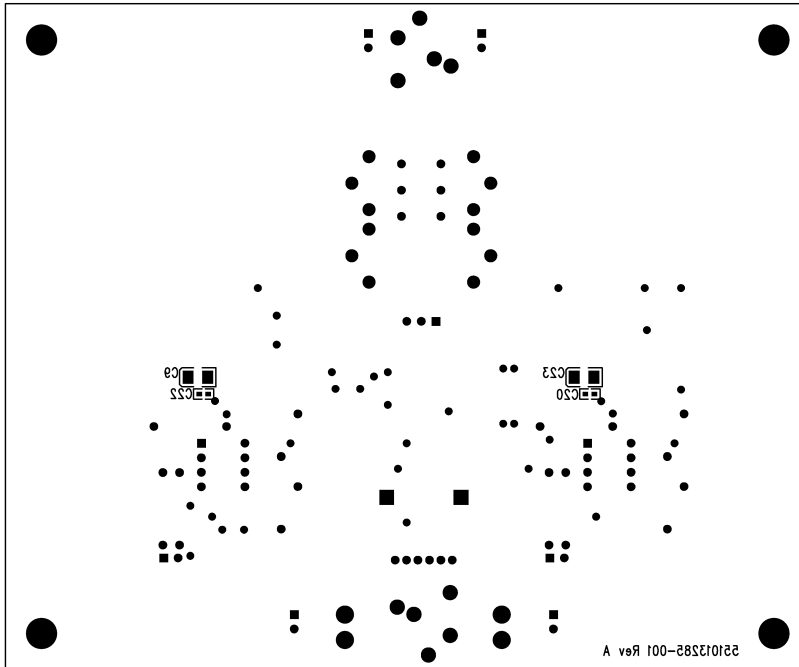
Figure 6. Bottom Silk Layer
