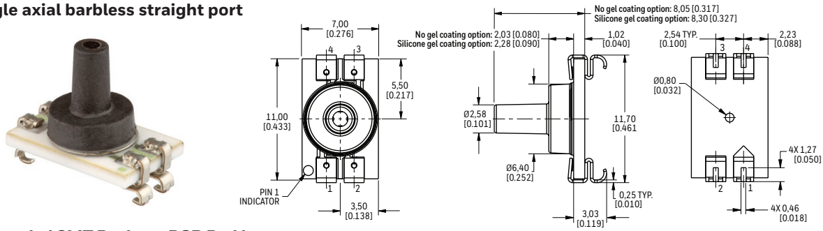
FIGURE 2. SMT PACKAGE DIMENSIONAL DRAWINGS (FOR REFERENCE ONLY: MM [IN], CONTINUED.)
