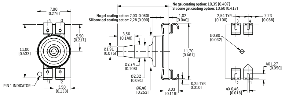
FIGURE 2. SMT PACKAGE DIMENSIONAL DRAWINGS (FOR REFERENCE ONLY: MM [IN].)
