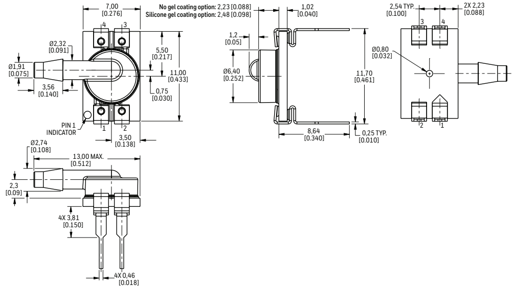
FIGURE 1. DIP PACKAGE DIMENSIONAL DRAWINGS (FOR REFERENCE ONLY: MM [IN], CONTINUED.)
