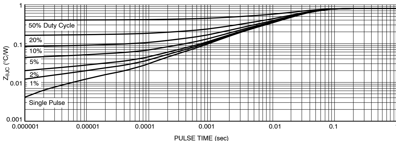
Figure 13. Thermal Impedance
