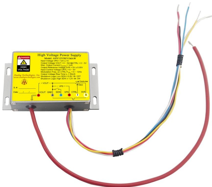
Figure 1.1. Top View of AHV12V5KV1MAW
