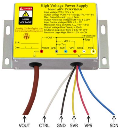
Figure 2. The Connecting Lead Wires of AHV12V5KV1MAW
