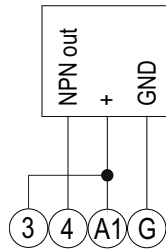
Fig. 15 NPN impulse input (product code: 2TCW)
