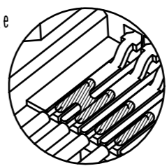
Solder bridge
