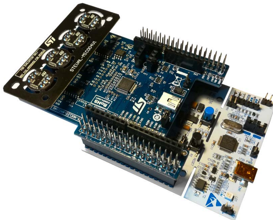
Figure 2. X-NUCLEO-AMICAM1, STM32 Nucleo and STEVAL-MIC004V1 stack
