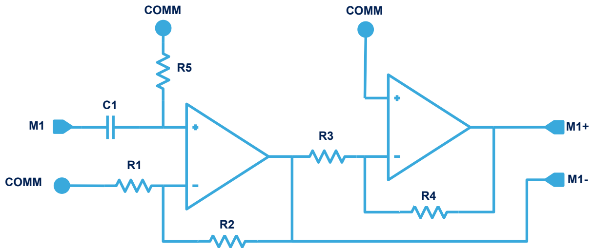
Figure 5. X-NUCLEO-AMICAM1 expansion board: amplification and conversion to differential
