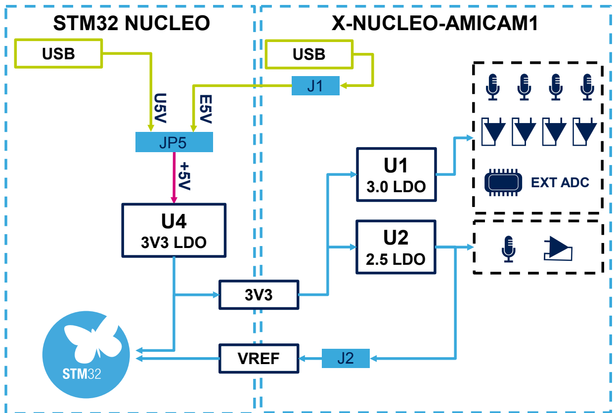
Figure 6. X-NUCLEO-AMICAM1 expansion board: power supply scheme
