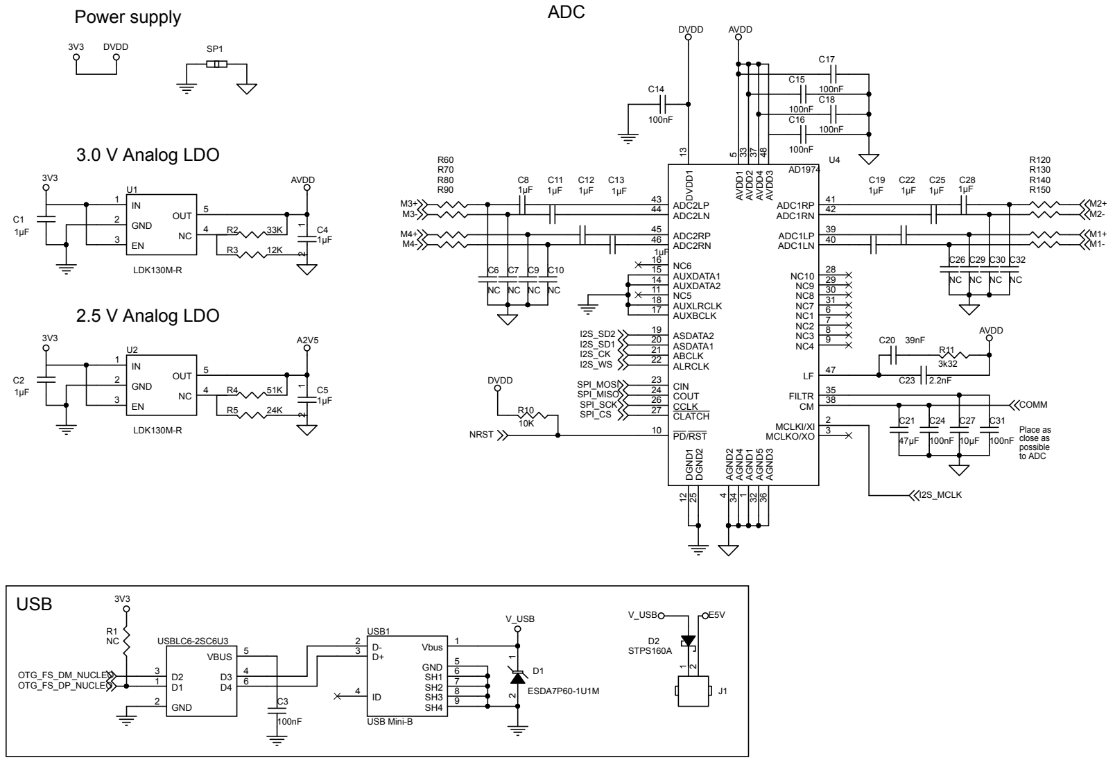
Figure 8. X-NUCLEO-AMICAM1 circuit schematic - USB, power, external ADC
