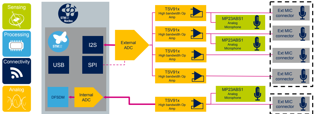
Figure 3. X-NUCLEO-AMICAM1 expansion board block diagram
