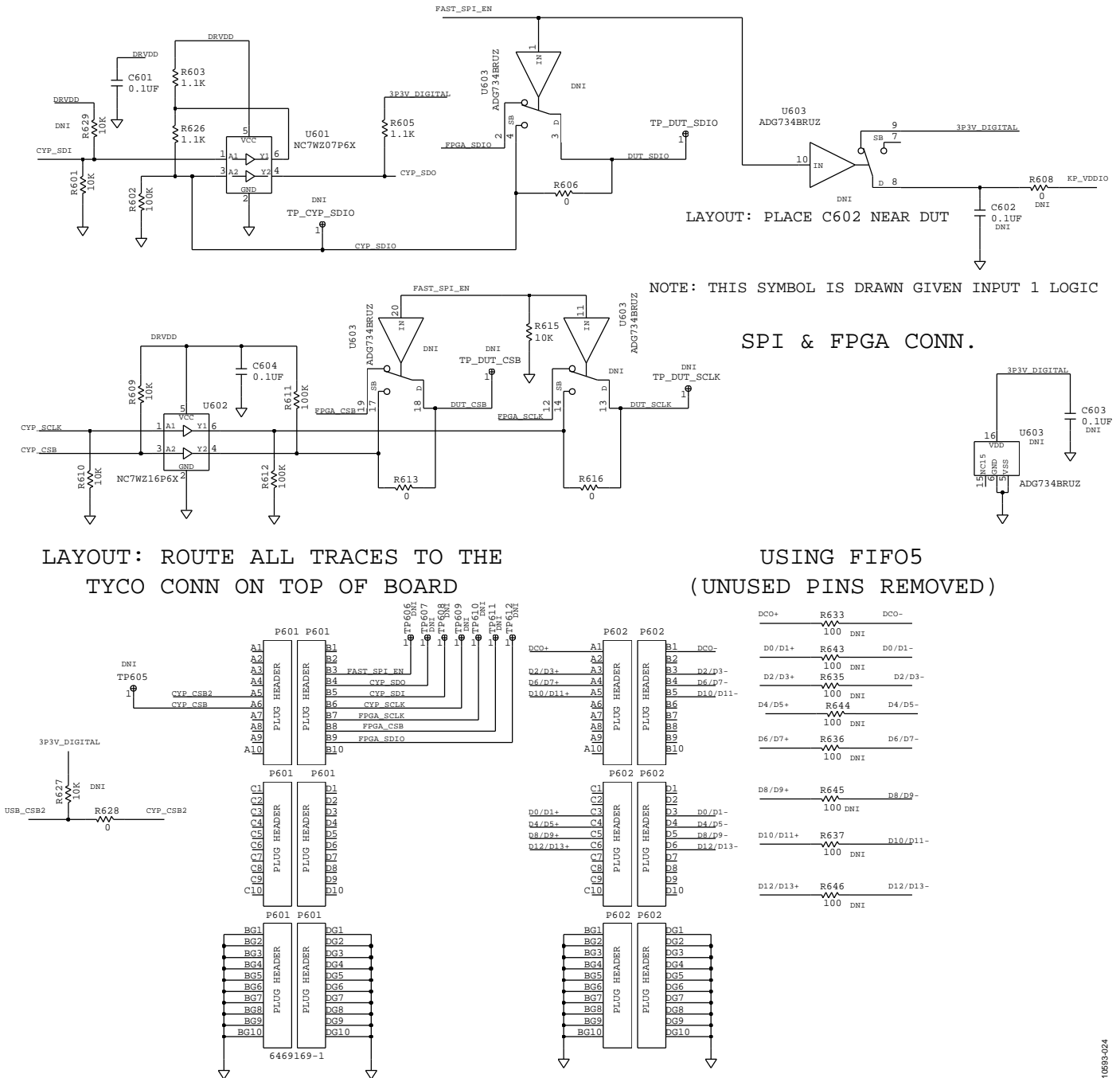
Figure 23. SPI Configuration Circuit and FIFO Board Connector Circuit
