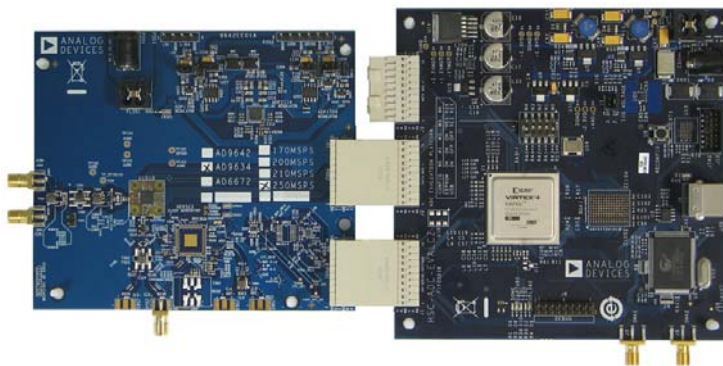
Figure 1. AD9642, AD9634, or AD6672 Evaluation Board (on Left) and HSC-ADC-EVALCZ Data Capture Board (on Right)
