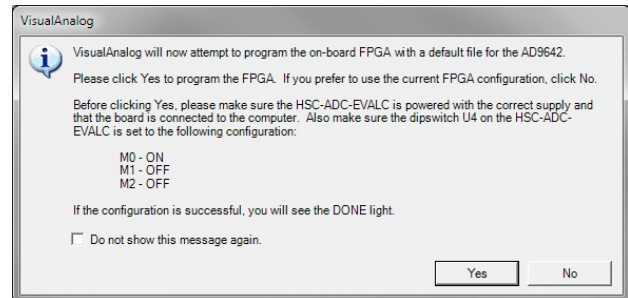
Figure 5. VisualAnalog Default Configuration Message
