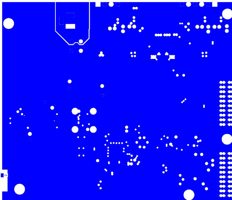
Figure 25. Ground Plane (Layer 2)
