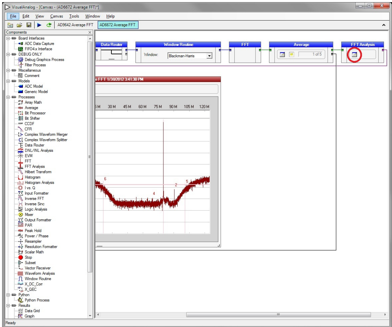
Figure 15. VisualAnalog, Main Window—Showing FFT Analysis for AD6672
