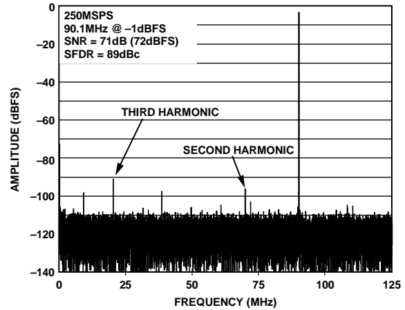
Figure 13. Typical FFT, AD9642
