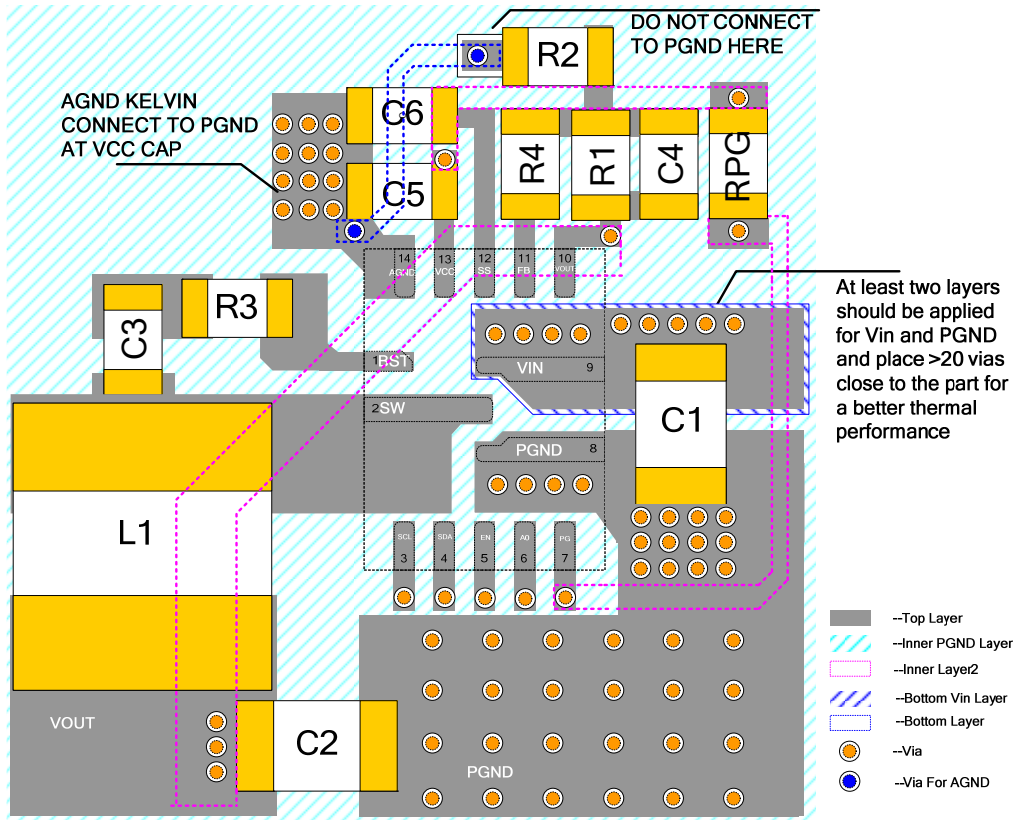
Figure 14: Recommended Layout
