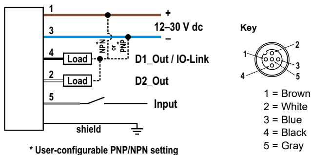
Figure 4: IO-Link Models
