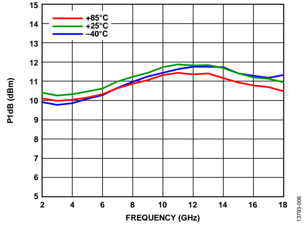
Figure 6. P1dB vs. Frequency for Various Temperatures
