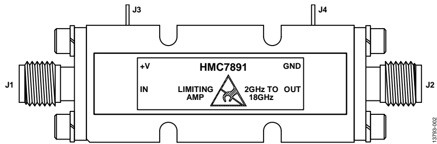
Figure 2. Pin Configuration
