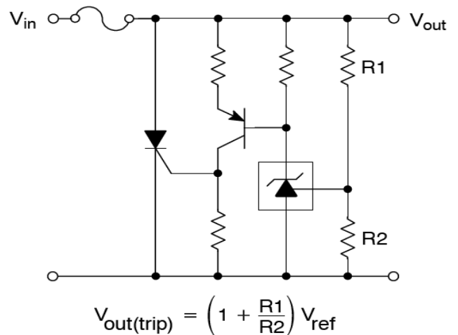
Figure 11: SCR Crowbar
