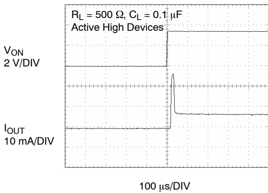
Figure 20. T_{ON} Response
