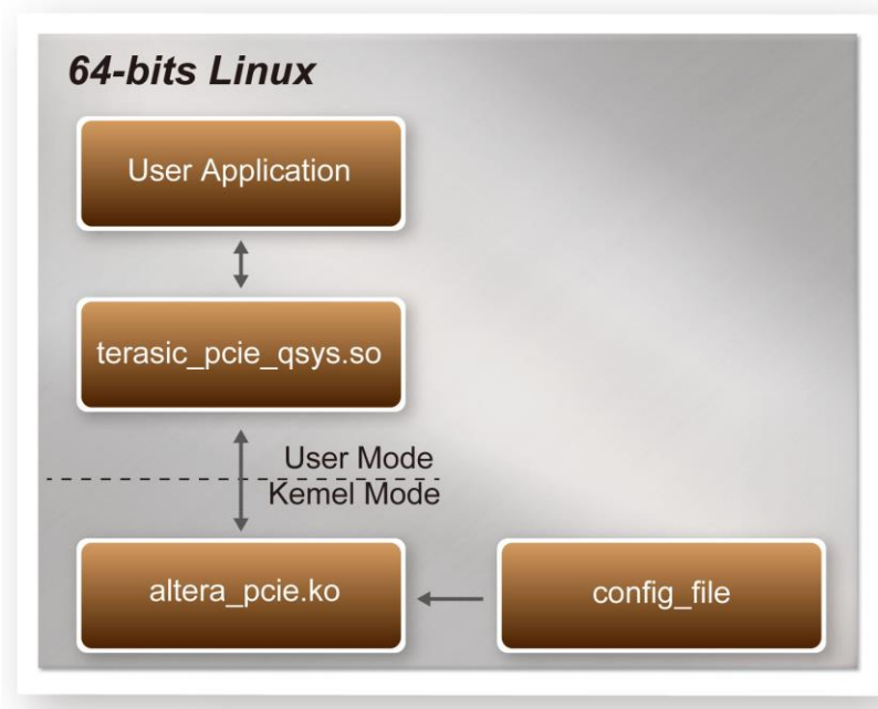
Figure 8-2 PCI Express Software Stack
