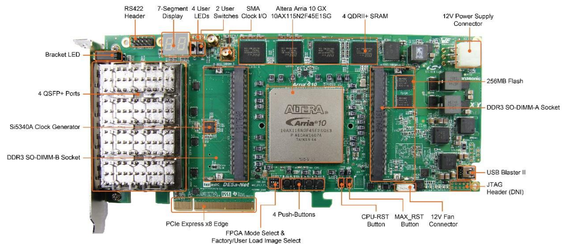
Figure 2-1 FPGA Board (Top)
