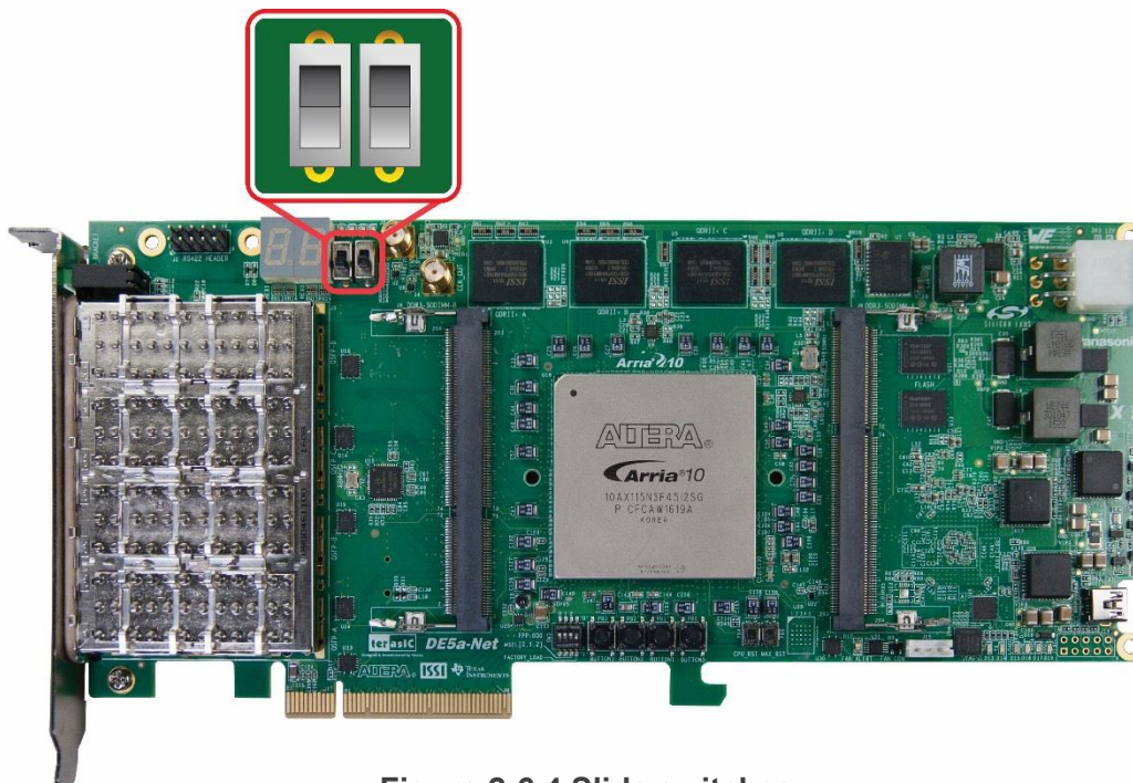
Figure 2-6 4 Slide switches
