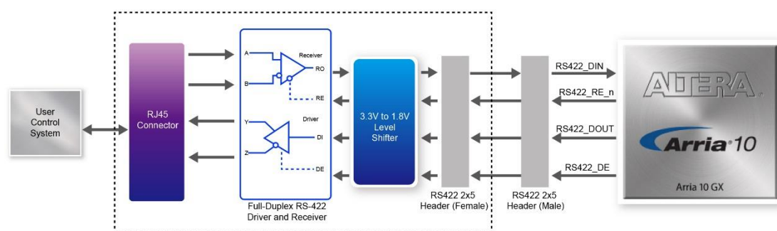
Figure 2-17 Block Diagram of RS-422 application
