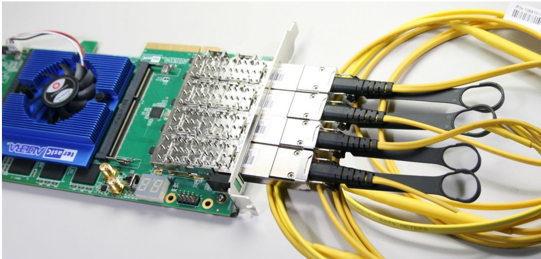
Figure 9-3 Two QSFP+ Cables Installed
