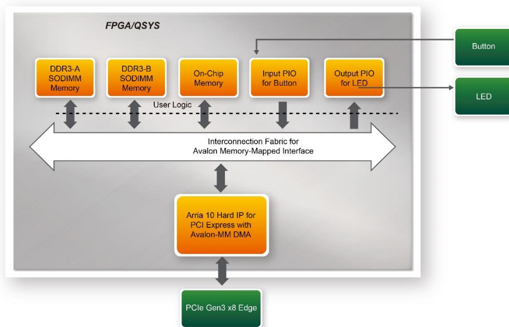
Figure 8-16 Hardware block diagram of the PCIe_DDR3 reference design
