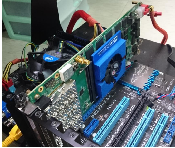
Figure 7-9 FPGA board installation on PC
