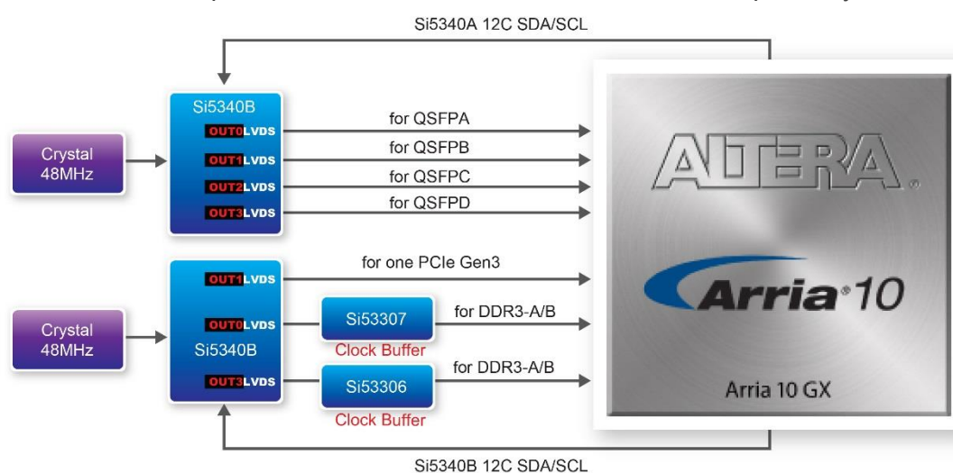
Figure 5- 2 Si570 Block diagram
