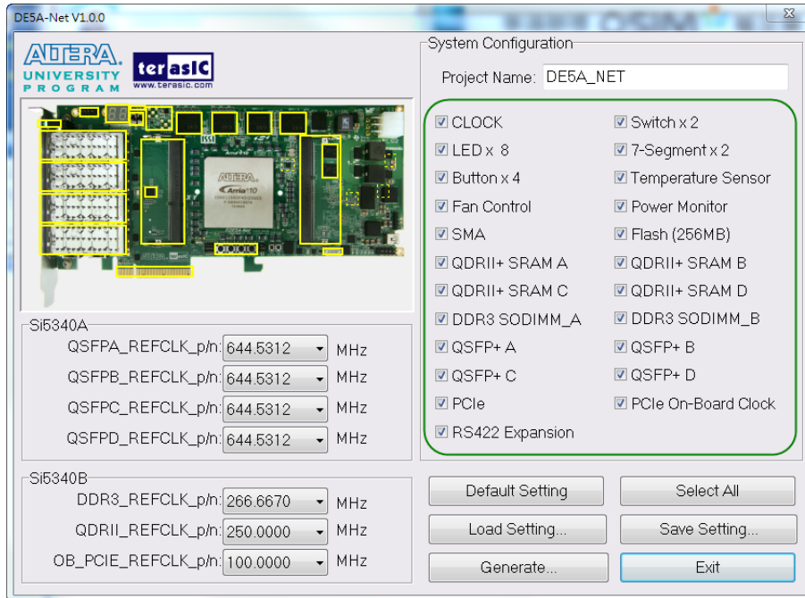
Figure 3-4 System Configuration group
