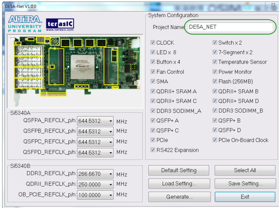
Figure 3-3 The Quartus project name
