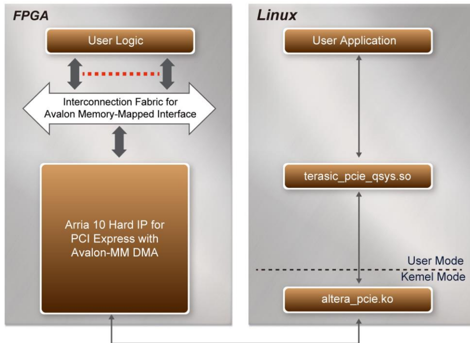
Figure 8-1 Infrastructure of PCI Express System
