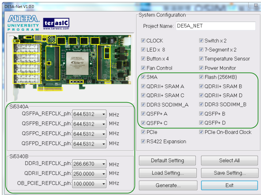
Figure 3-5 External programmable oscillators
