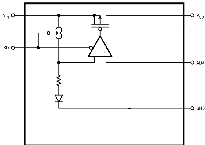
Figure 4. LP3855-ADJ
