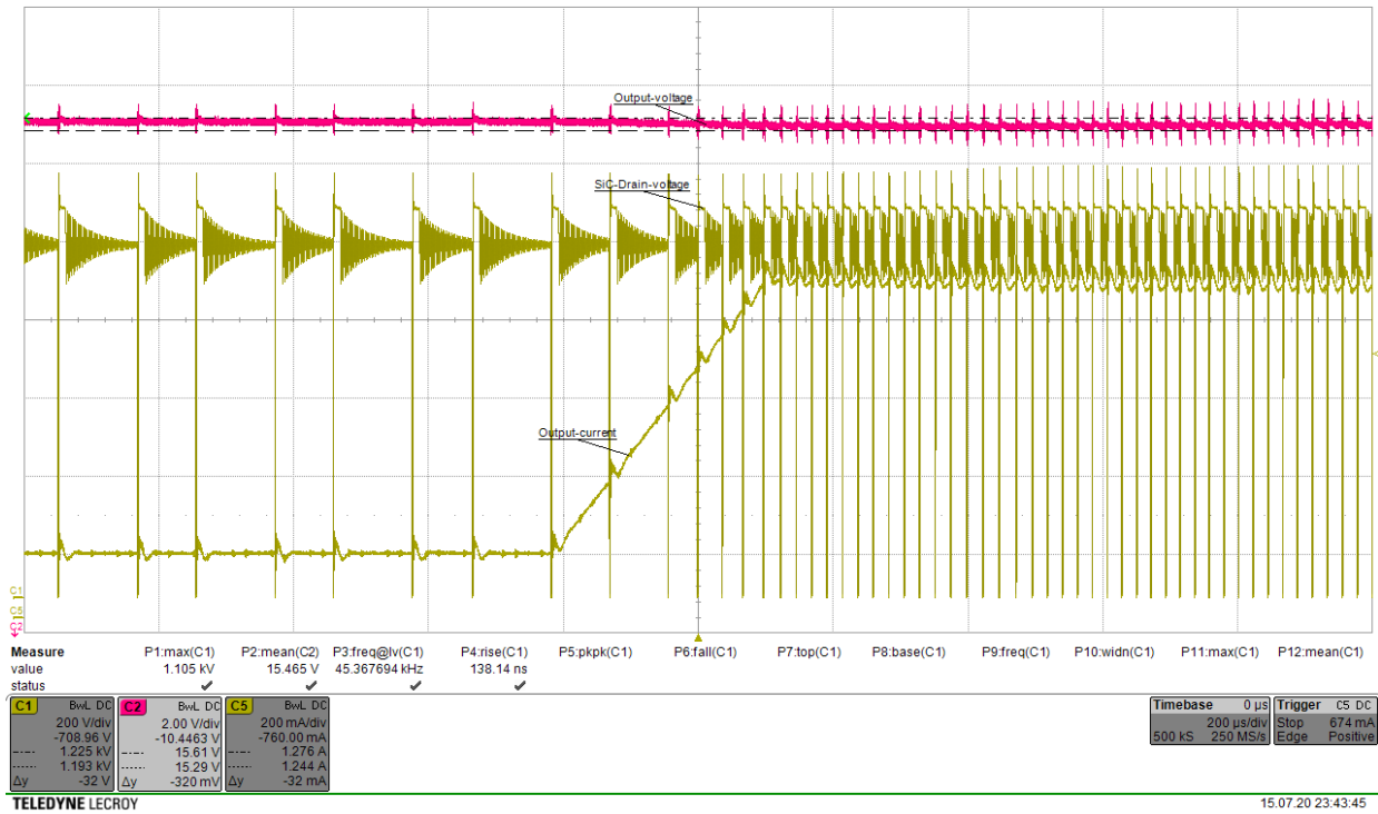
Figure 16. 900 V – 15% to 85%
